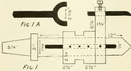
TOOL FOR TURNING TUMBLING SHAFTS.
